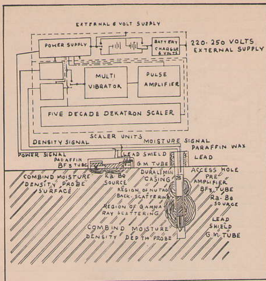
FIG. NO. 3 (1) & 4 (1) DIAGRAMMETRIC SKETCH OF MOISTURE-DENSITY APPARATUS
