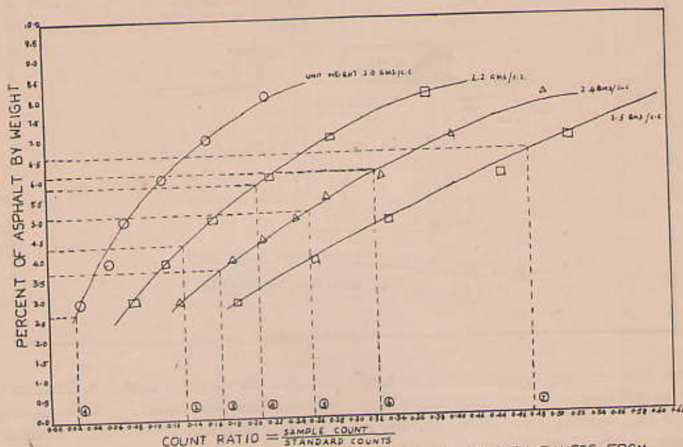
FIG. NO. 6 FINAL CALIBRATION CURVES FOR VARIOUS DENSITY RANGES FROM 2.0 GMS/c.c. TO 2.5 GMS/c.c. SAMPLE SIZE 11" x 11" x 2"
